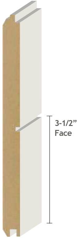
1x8 Reversible T&G Nickel Gap with V-Groove
